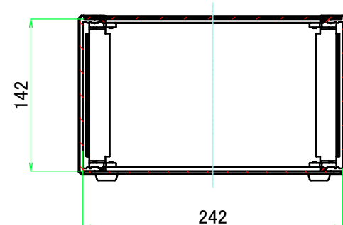
B-B (1:5)
